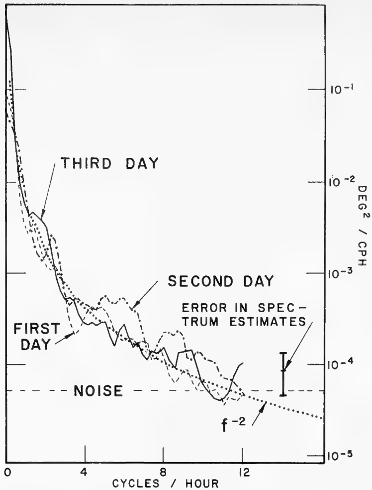
Figure 8. Spectral density estimates for the temperature records of three successive days, Buoy 2, at 150 ft.
